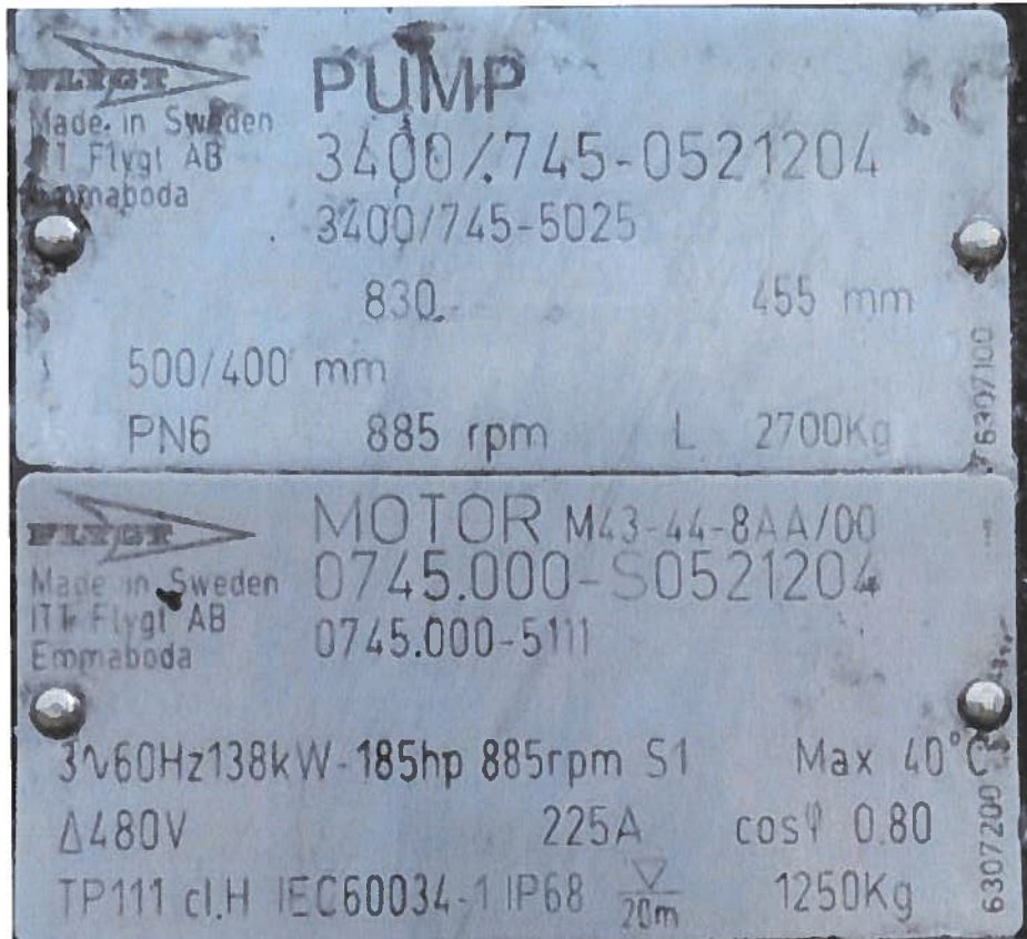
Figure 1 - Motor Name Plate Data for AFD 100, 200, 400
